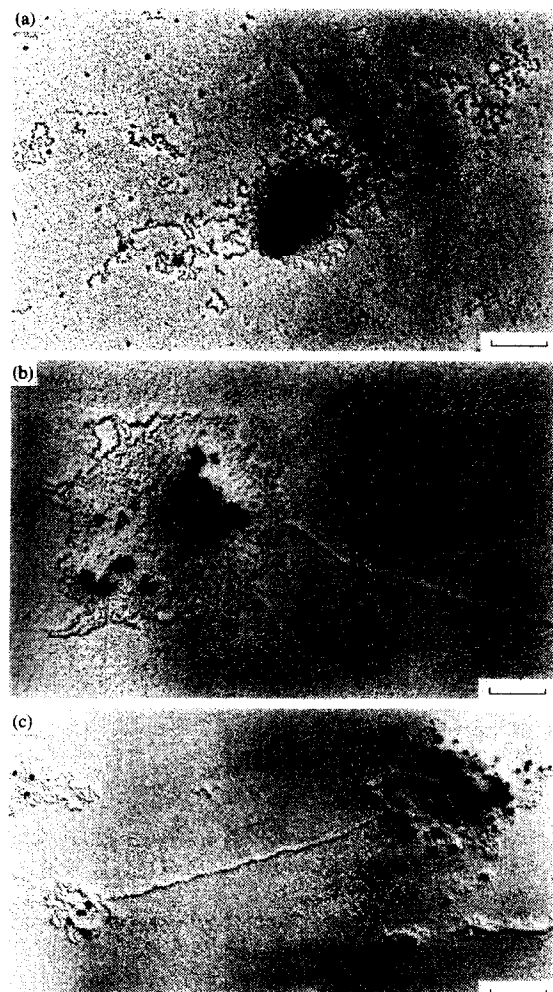
Fig. 7. Electron micrographs of (a) pig gastric mucin complexed with chitosan labelled with WGA-Au 10 (PGM-(SC-WGA-Au 10 ), Table 3), (b) pig gastric mucin complexed with chitosan-colloidal gold conjugates using chitosan SC210 (PGM-(SC-Au 4 ), Table 3), and (c) chitosan KN50 (PGM-(KN50-Au 4 ), Table 3). The scale bar is 200 nm.
